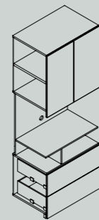
Modulo porta Tv fisso L 878/1178 W878/1178 Tv module with fixed back panel
