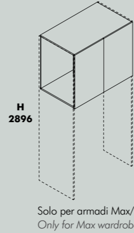
Moduli sopra porta L 1178 P. 494/498/592/596 W1178 Over door modules D.494/498/592/596
