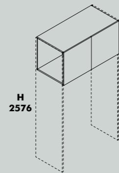
Moduli sopra porta L 1178 P. 494/498/592/596 W1178 Over door modules D.494/498/592/596
