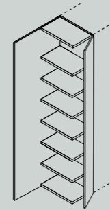
COVER 494/498/ 592/596 Anta con 7 ripiani Door and 7 shelves
