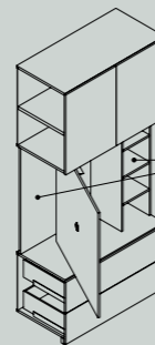
Modulo porta Tv girevole L 878/1178 W878/1178 Tv module with swivel back panel
